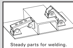
Steady parts for welding.
